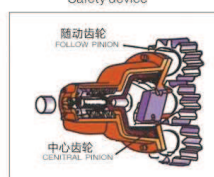
防坠安全锁 Safety device
