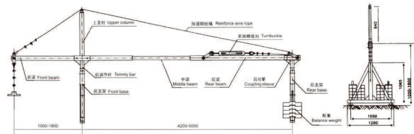
ZLP系列悬挂机构名称及规格 ZLP series high operation suspending part name and size
